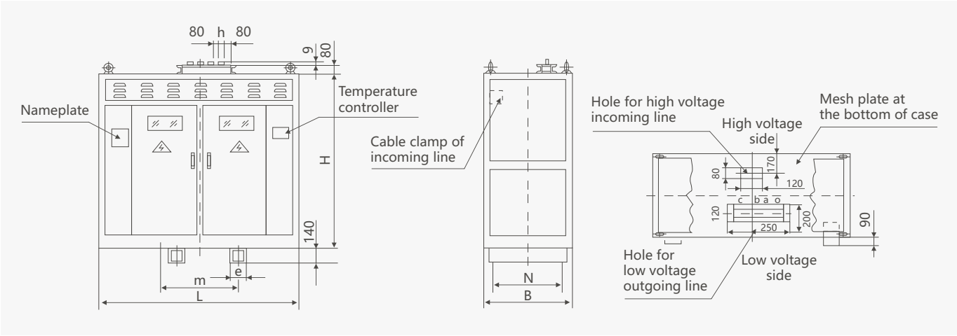
Outline diagram of IP20 of SG(B)10 type non-encapsulated coil power transformer (HS3)
