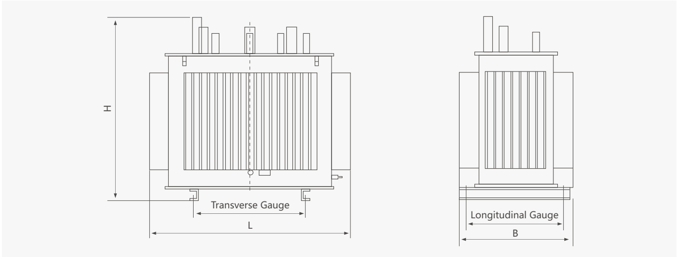
Overall and mounting dimensions(mm)
