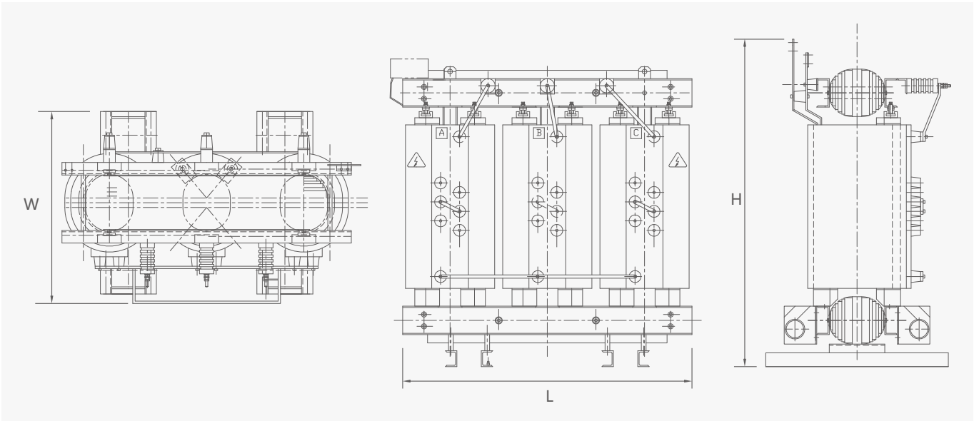
Overall and mounting dimensions(mm)
